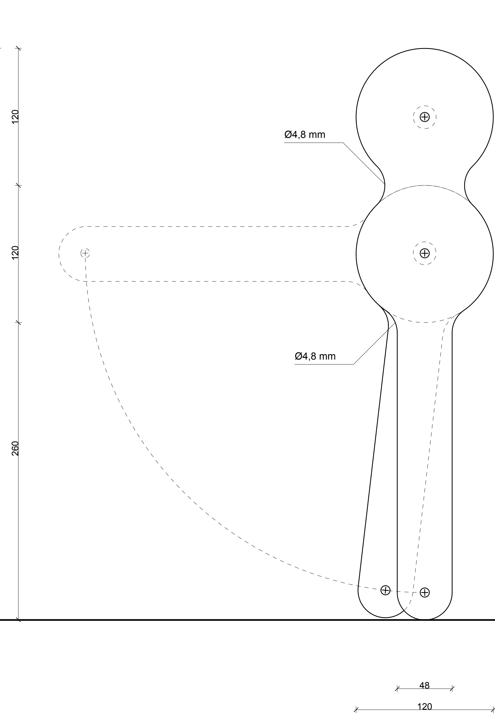
SIDE VIEW
