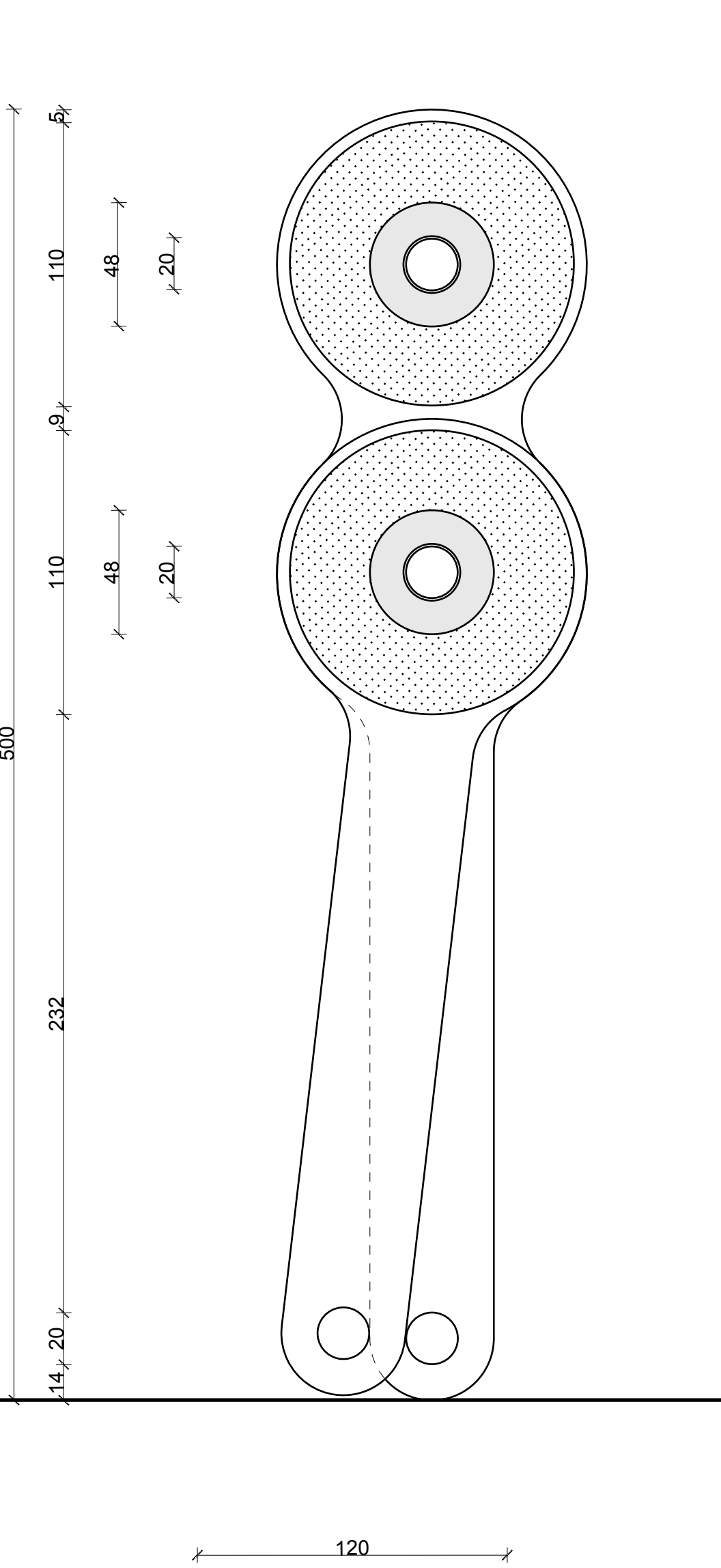
CROSS-SECTION A-A
