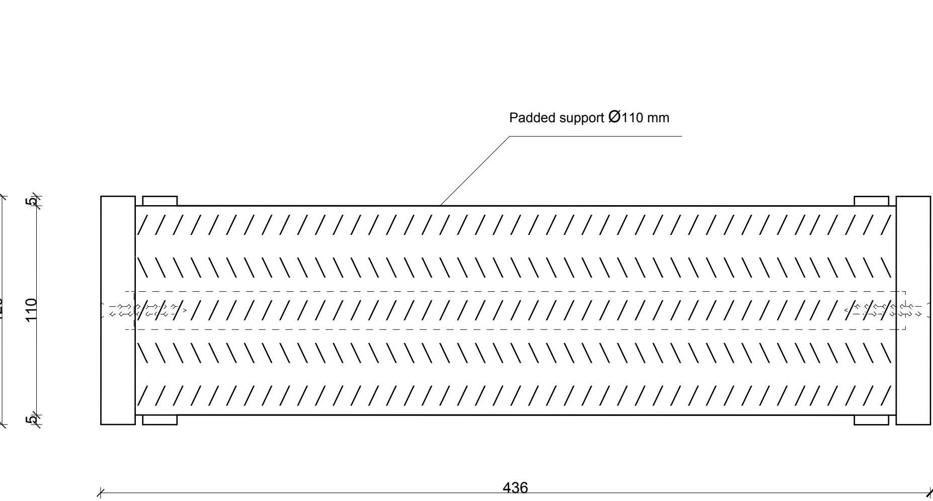
TOP VIEW
