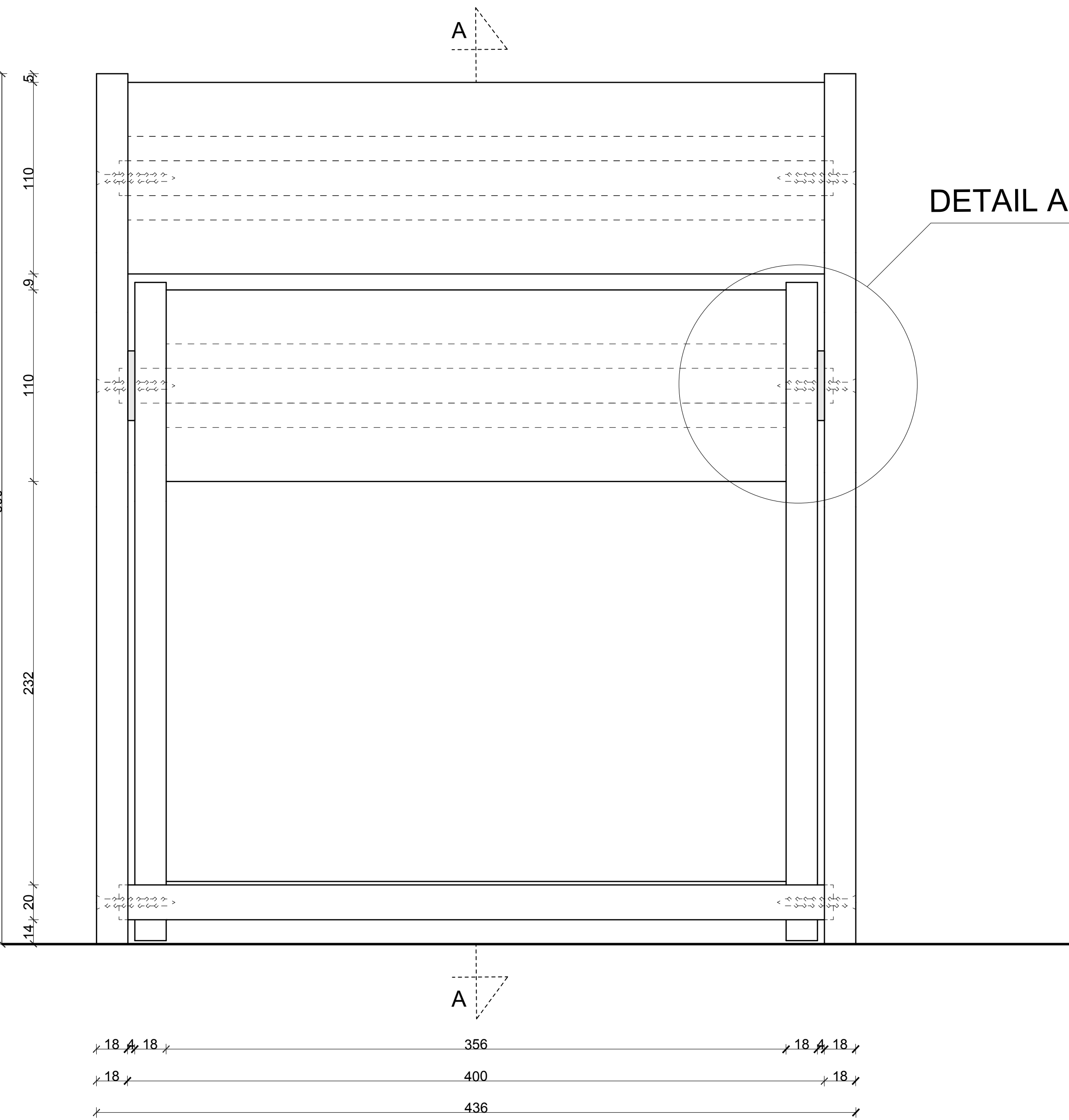
FRONT VIEW
